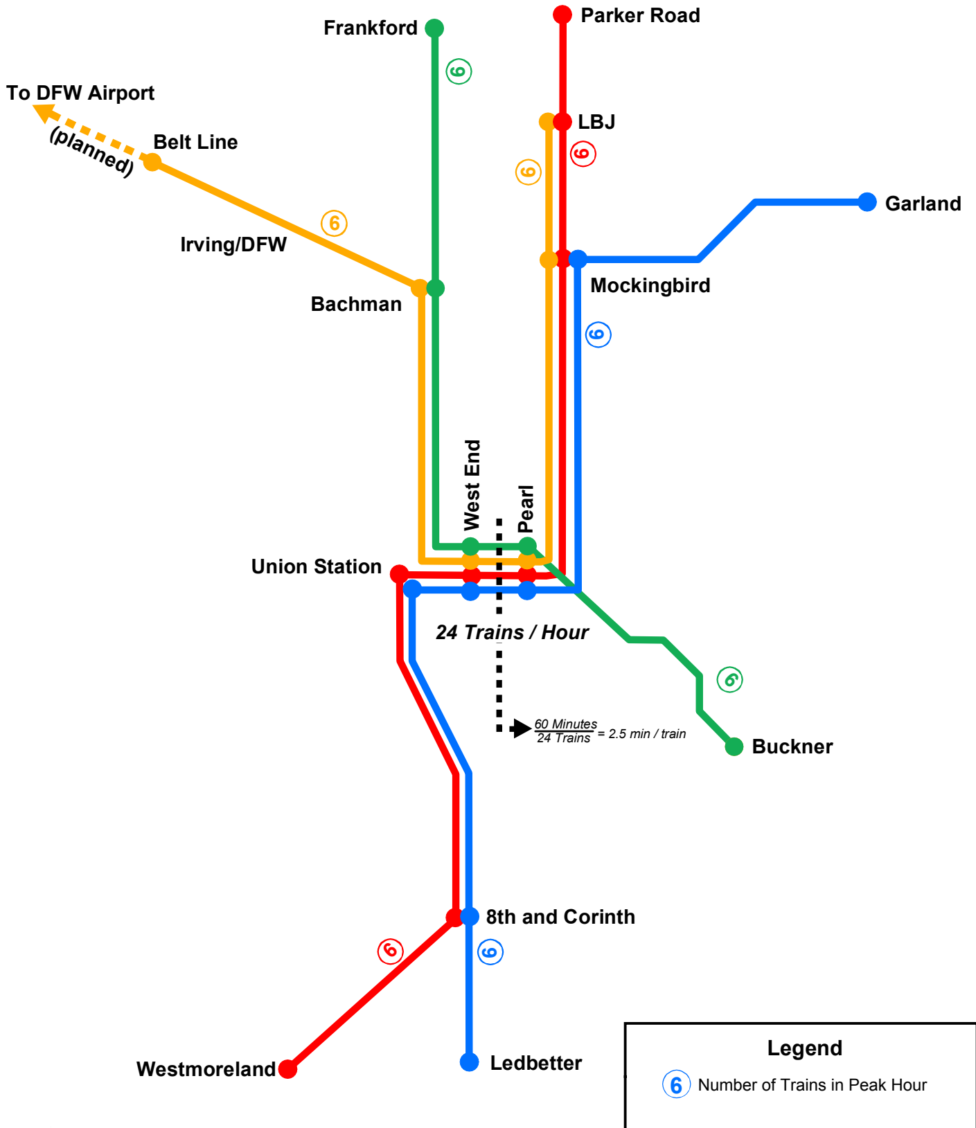
Figure 2-18 LRT Alternative Rail Operating Plan
